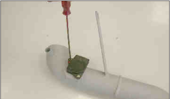
25. Install the stock mass air sensor into the K&N® cold air tube and secure with the provided hardware as shown.
