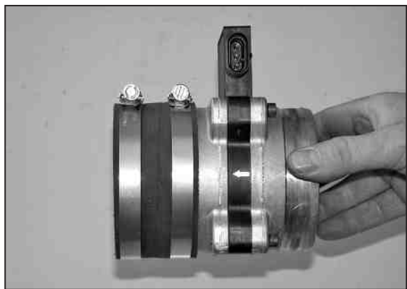
27. Install the silicone hose (#08698) onto the intake tube side of the mass air sensor and secure with the provided hose clamp. NOTE: There is an arrow on the side of the mass air sensor which shows direction of air flow through the sensor and points the intake tube side of the sensor.
