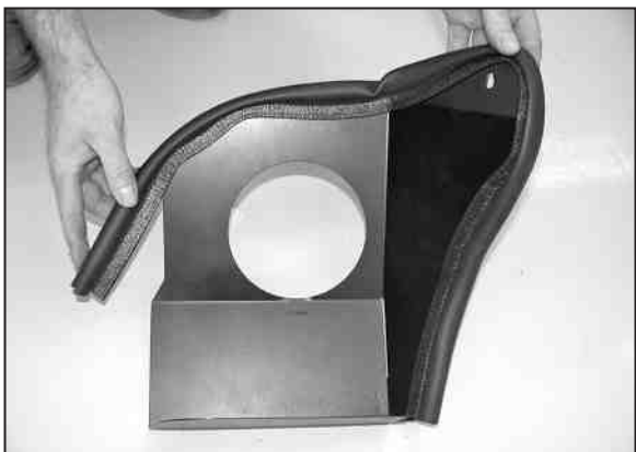
18. Install the provided edge trim onto the heat shield as shown.
