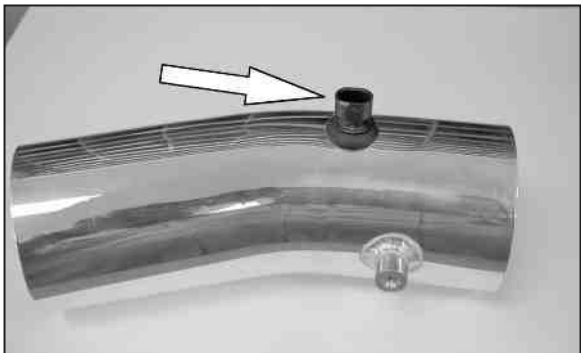
16. Install the air temperature sensor from step #15 into the grommet in the K&N® intake tube as shown.
