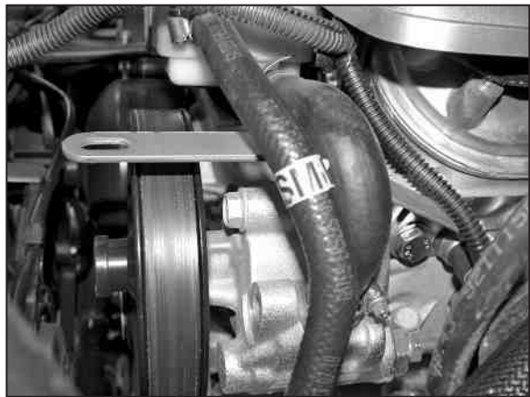
12. Install the tube bracket #010076 using the provided hardware. NOTE: The 10mm mounting bolt threads into the threaded, unused hole in the cylinder next to coolant temperature sensor.
