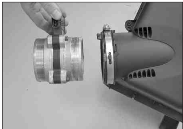
26. Loosen the hose clamp that secures the mass air sensor to the factory air box, then remove the mass air sensor from the factory air box.
