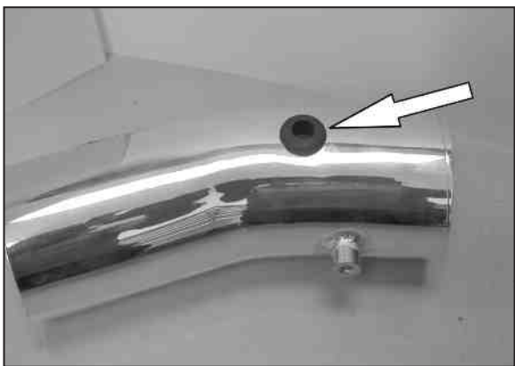
15. Install the provided rubber grommet into the K&N® intake tube as shown. NOTE: Before installing the rubber grommet, inspect the inside of the tube for any debris, then clean the inside out with water and a towel. Inspect the tube one more time before proceeding to the next step.
