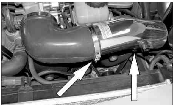
17. Install the K&N® intake tube onto the throttle body silicone hose and tighten hose clamp but not completely. Align the bracket installed in step #12 to the bung on the intake tube and tighten using the hardware provided.
