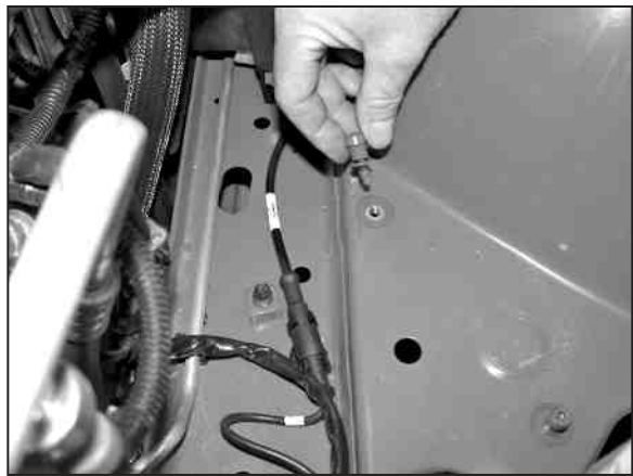
11. Remove the inner air box mounting stud shown with a T-30 torx socket.
