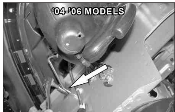
13. Remove the two bolts that secure the air intake resonator as shown. On '04-'06 models, refer to photos above as to locations of bolts.
