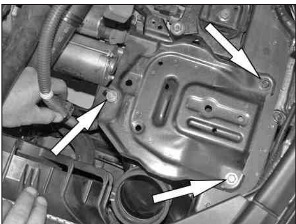
20. Unclip the battery cable from the battery tray, then, remove the two top bolts and loosen the two lower bolts that secure the battery tray to the inner fender.
