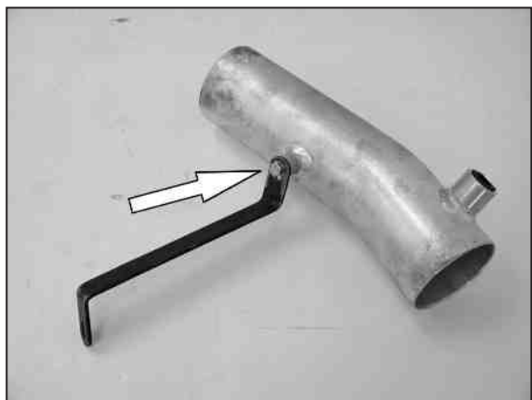
27. Secure the provided "Z" bracket to the K&N short ram tube using the provided hardware as shown. NOTE: Before securing the "Z" bracket, inspect the inside of the tube for any debris, then clean the inside out with water and a towel. Inspect the tube one more time before proceeding to the next step.
