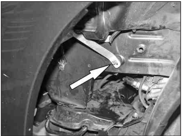
35. Secure the bracket on the cold air tube to the rubber mounted stud from step 33 using the provided hardware as shown.
