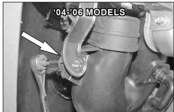
17. Loosen and remove the battery hold down bracket as shown.
