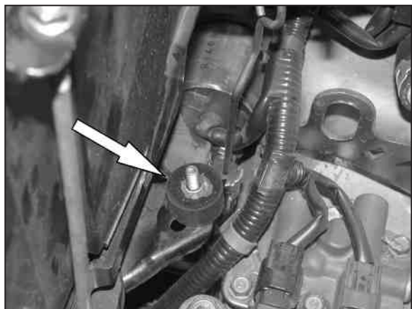
26. Install the rubber mounted stud into the original air cleaner mounting hole located directly behind the battery as shown.
