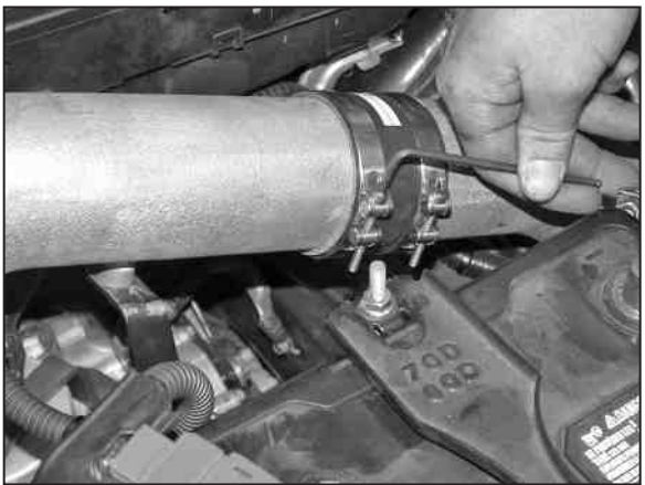
37. Align the tubes for best fit and clearance and tighten the hose clamps.
