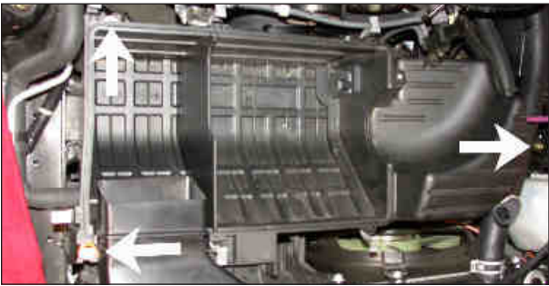
9. Remove the three bolts that secure the lower air cleaner assembly as shown.
