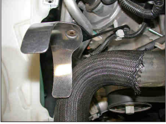
14. Install the wiring harness retaining clip removed in step #11 into the new tube mounting bracket, and then rescuer the wire harness to the clip as shown.
